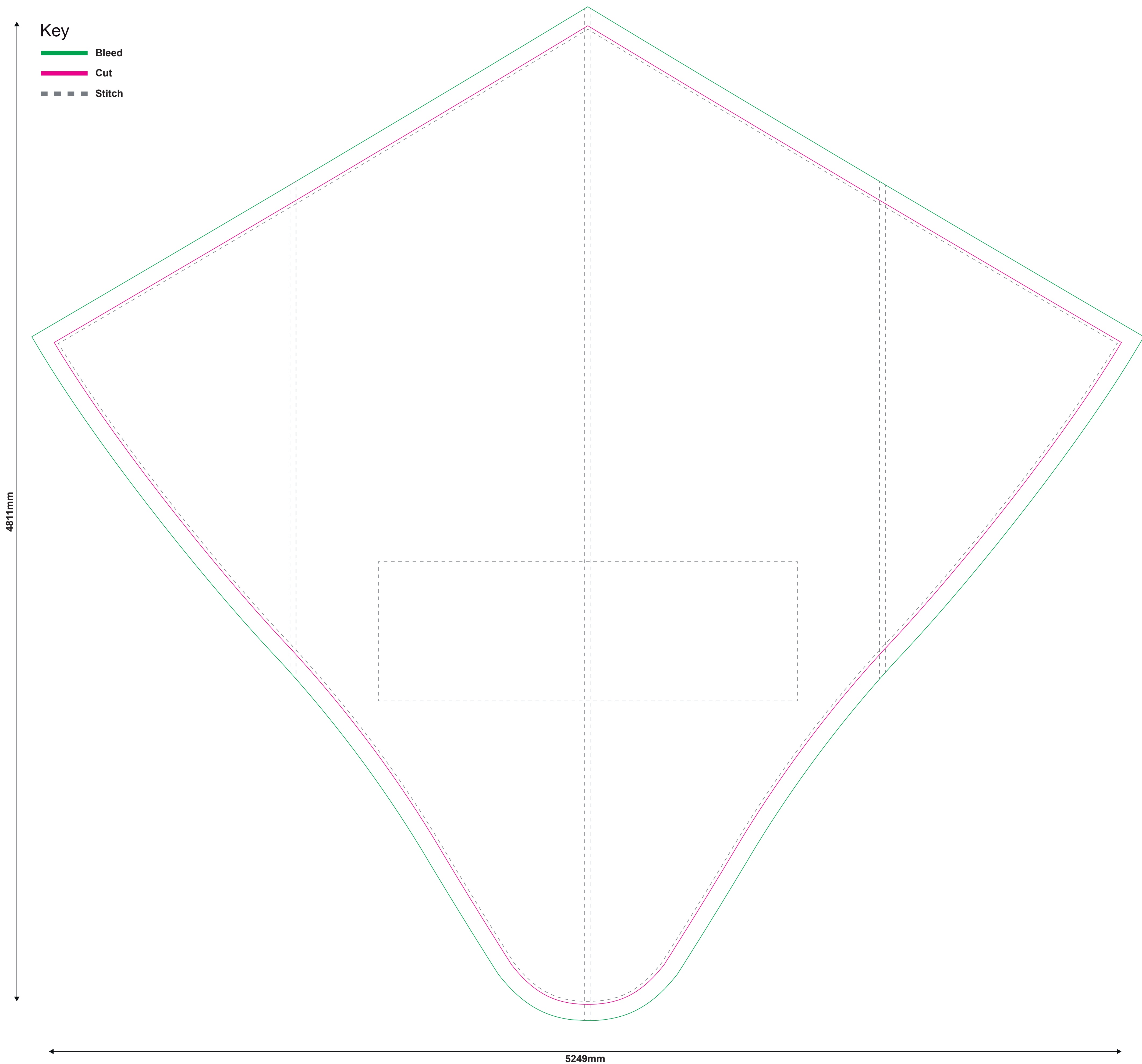
ROOF PANEL
